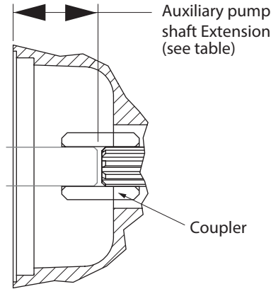
Auxiliary mount without charge pump
